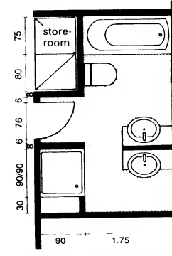
⑱ Bath and shower with separate washing area
